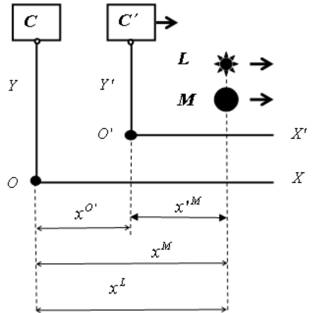
Figure 1. Coordinate representation of moving material points L , M , and O' in the inertial systems XOY and X'O'Y' . Systems XOY and X'O'Y' represent "resting" and "moving" systems, respectively; x are coordinates of points.
