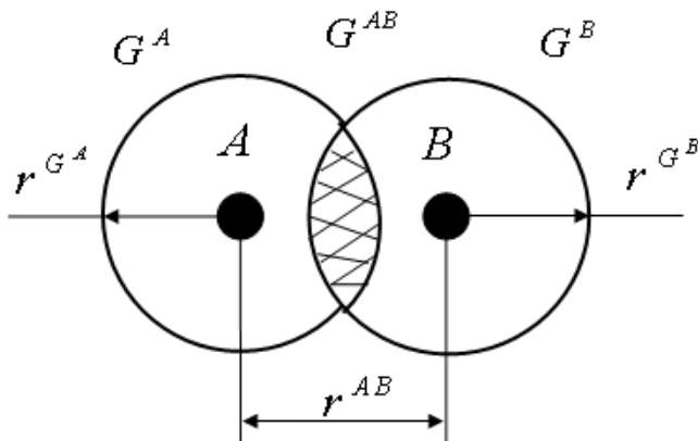
Figure 3. The gravitational interaction of the
